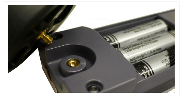
Mounting feature
